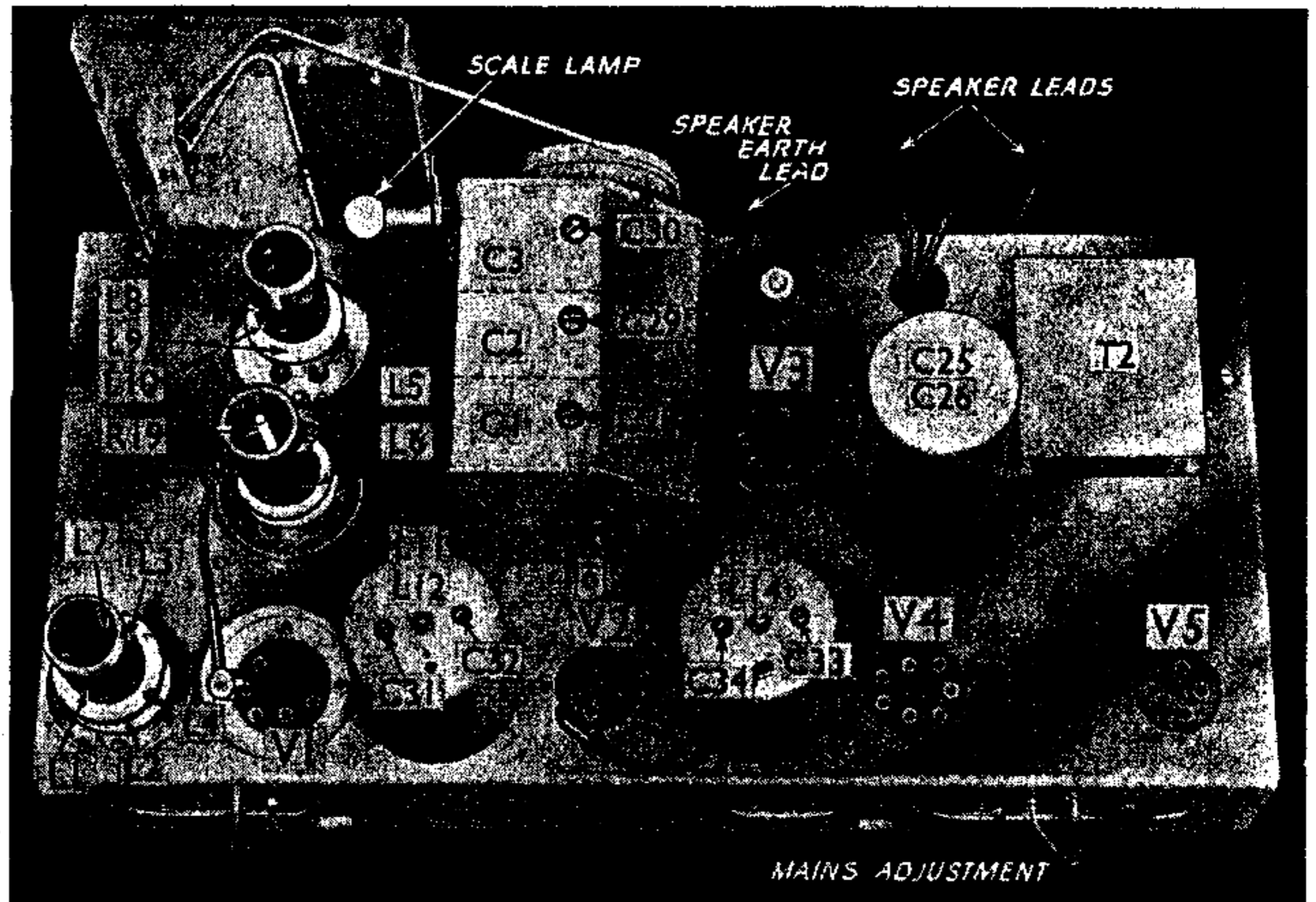
Plan view of the chassis. All the aerial and oscillator coil screens have been removed for photographic purposes. L7 can be seen in the L1-L4 unit, and R19 is indicated in the L5, L6 unit. The adjustment for L7 projects through the top of the screening can, and the coil is actually supported by the can, although it has been detached from the can and fitted in its normal position in the coil unit for photographing.
